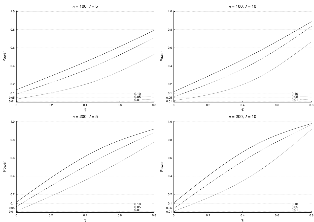
Figura 1: Hausman-type specification test for endogeneity: longitudinal data scenario
