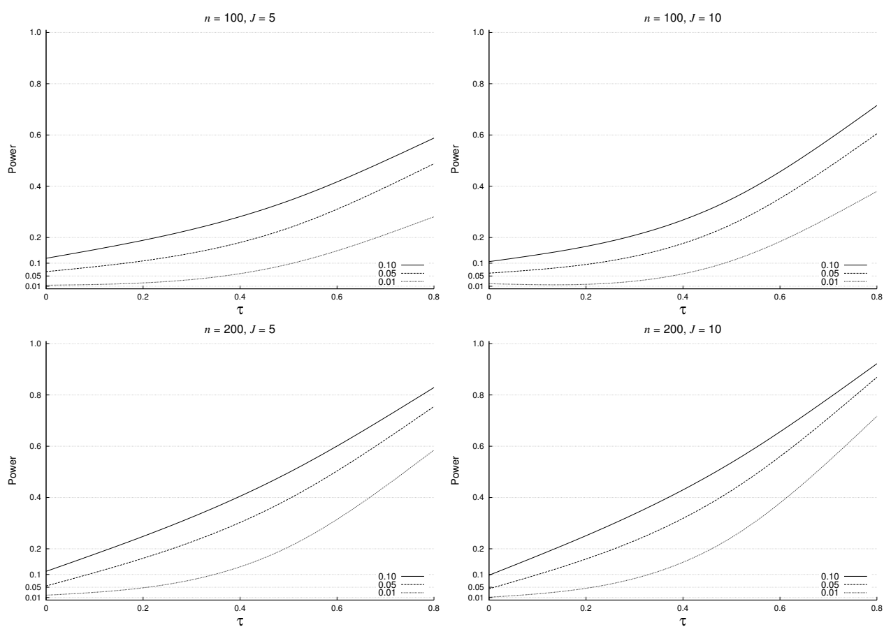
Figura 2: Hausman-type specification test for endogeneity: Rasch model scenario
